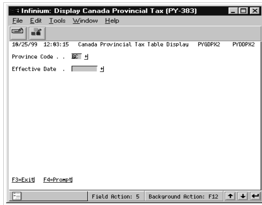
Figure 13-9: Canada Provincial Tax Table Display prompt screen
